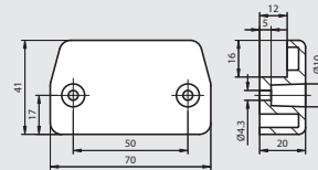
Holder for enabling switch
