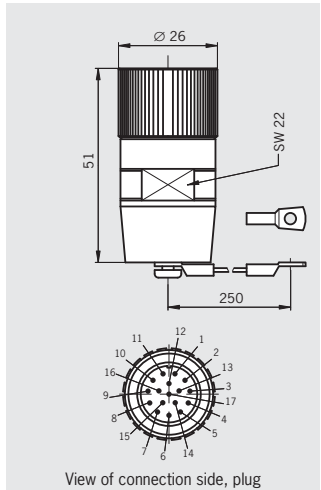
Blanking plug RC17 17-pin
